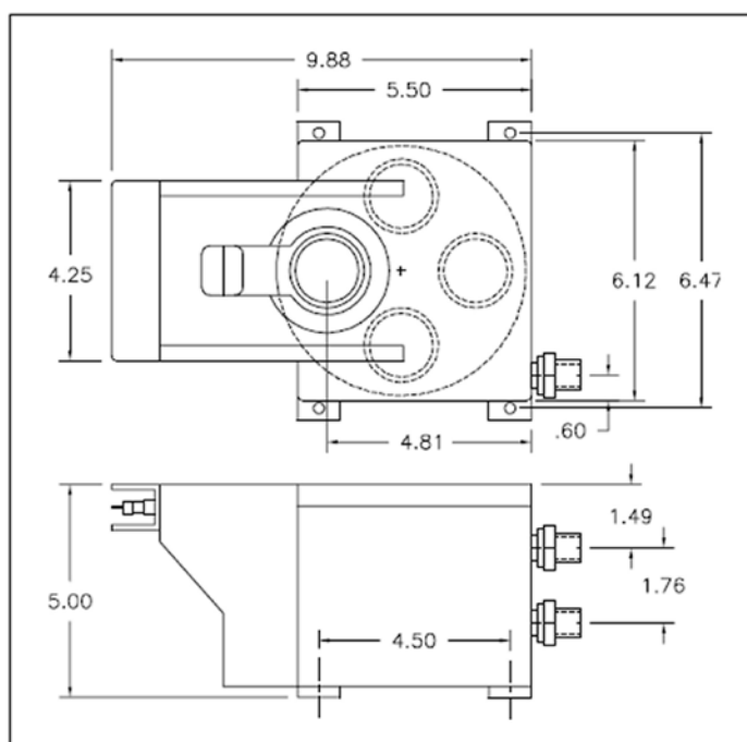
FIG. 1 - HCR Rotary E-Gun dimensional outline
